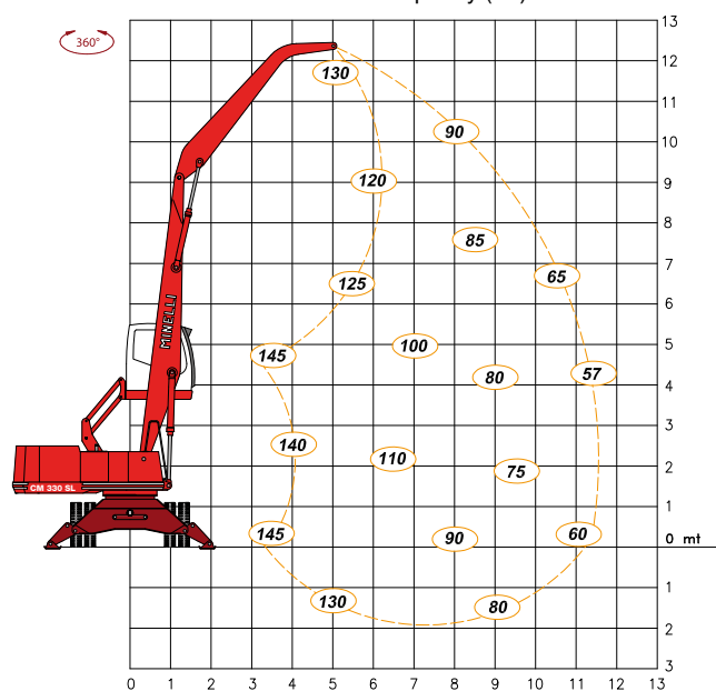
Stabilised machine load capacity (kN)
